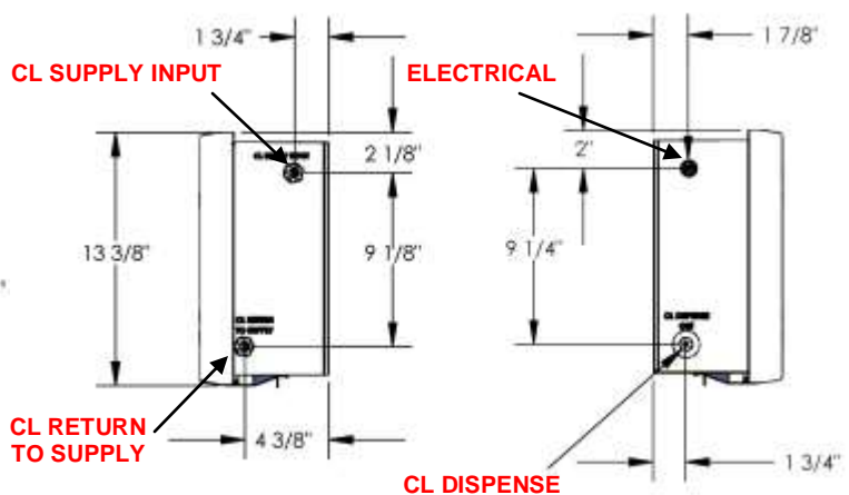
Diagram 2 (Right Side)
